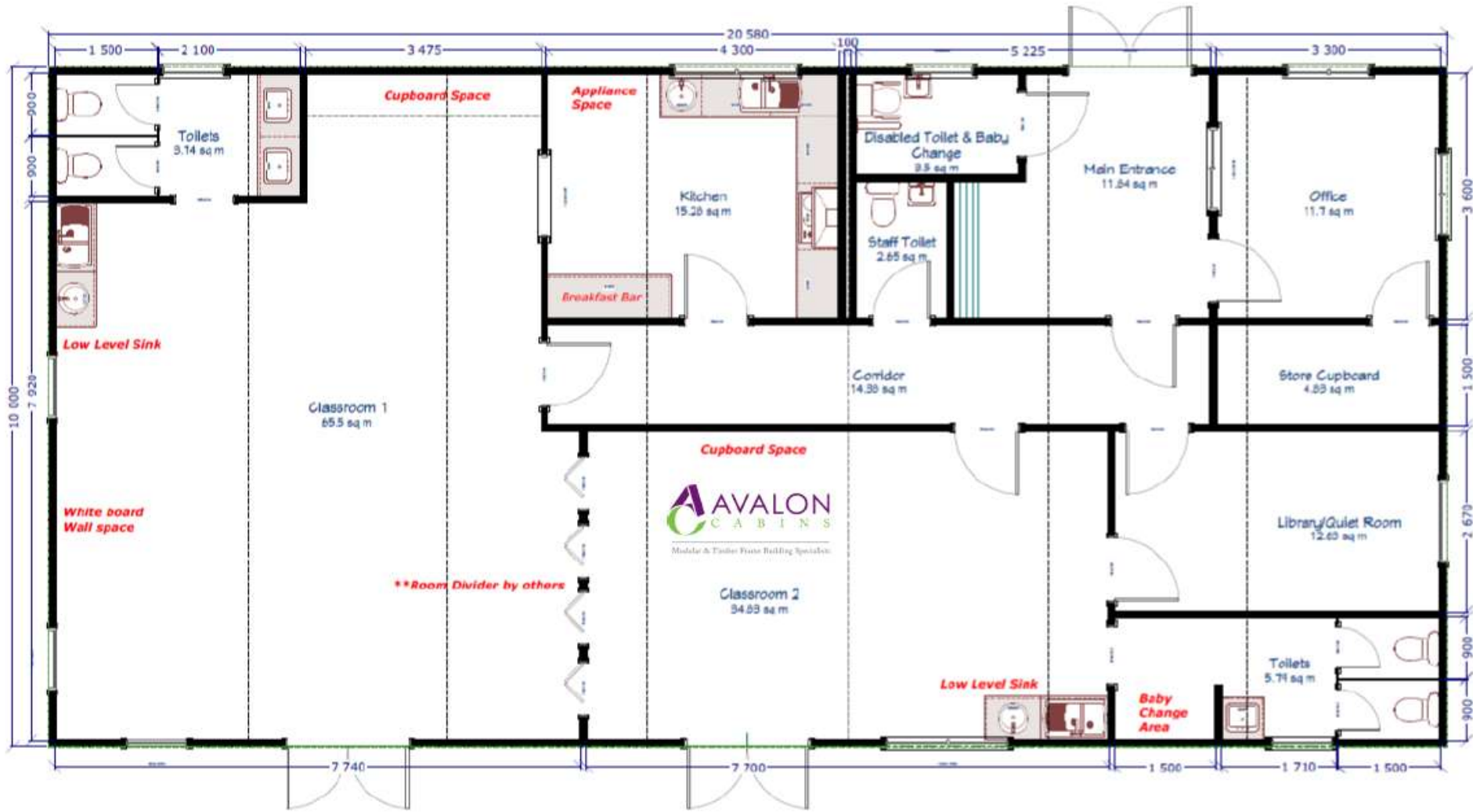
PROPOSED NEW BUILDING FLOOR PLAN
